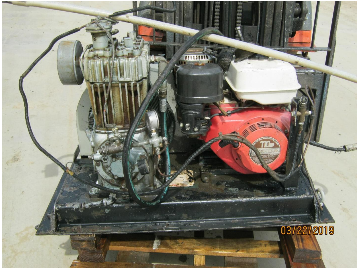
HONDA POWER COMPRESSOR
